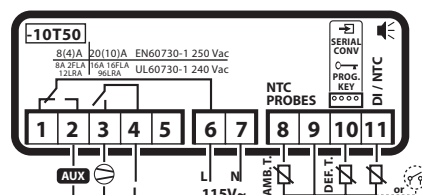
Two Relay Wiring Diagram (Diagram No. 2)
