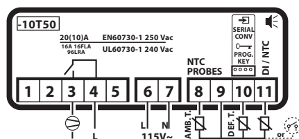
One Relay Wiring Diagram (Diagram No. 1)
