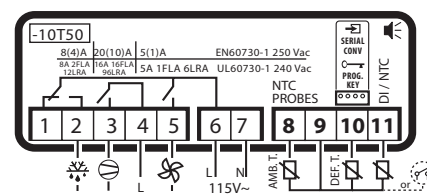
Three Relay Wiring Diagram (Diagram No. 3)
